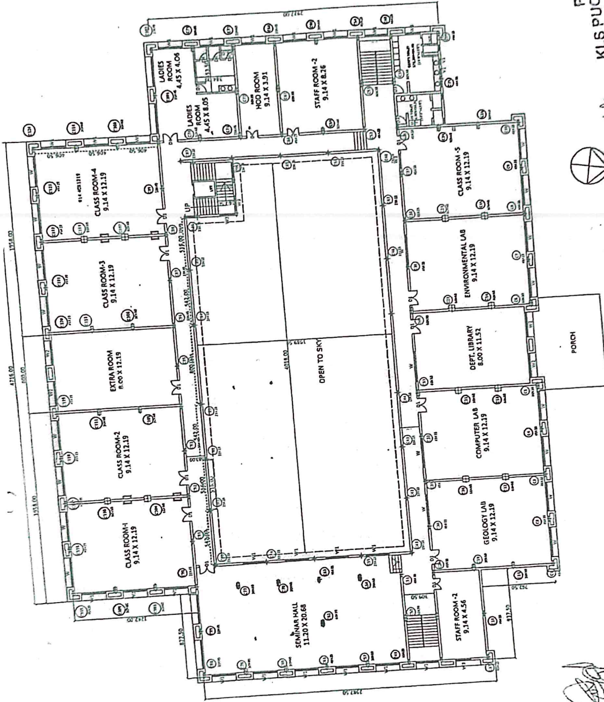
SECOND FLOOR PLAN ALT. -1
